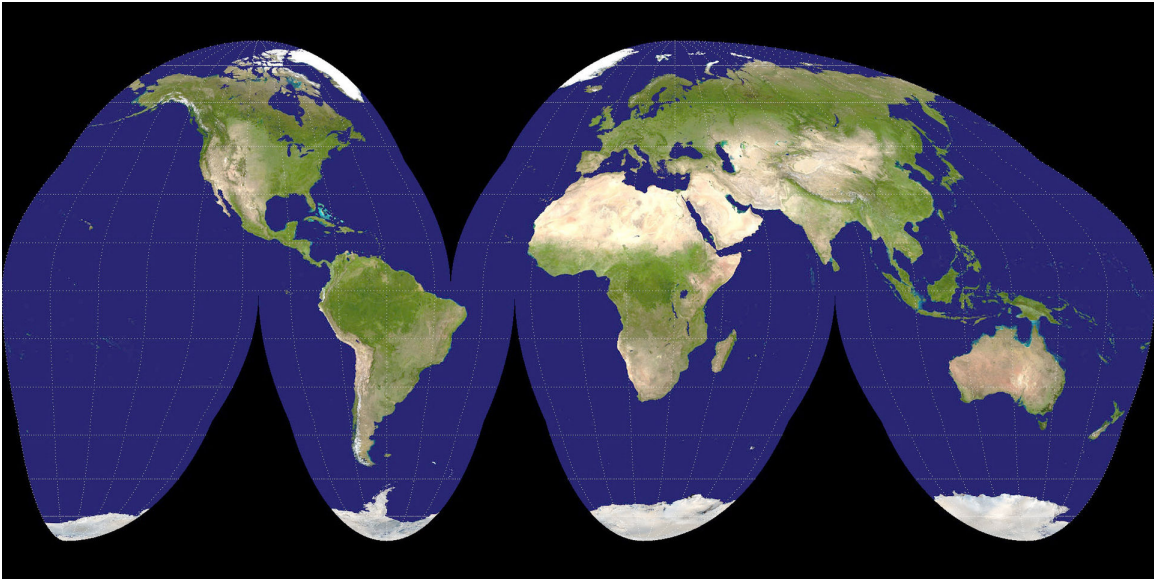
A Goode projection of a Visible Earth image collected by the Earth Observatory experiment of the U.S. Government's NASA space agency. Photo: Wikimedia.
